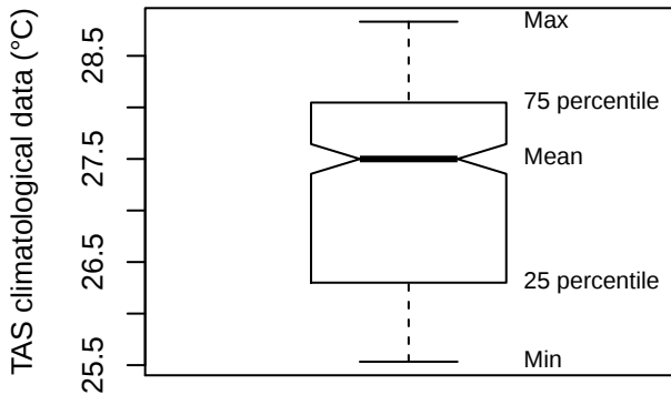
Box plot (TRTC)
