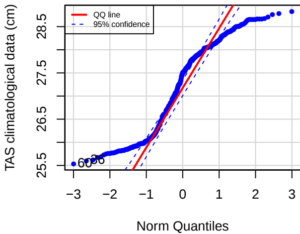
QQ plot (TRTC)
