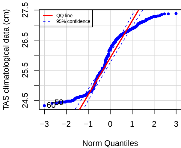
QQ plot (TRTR)
