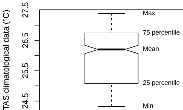
Box plot (TRTR)
