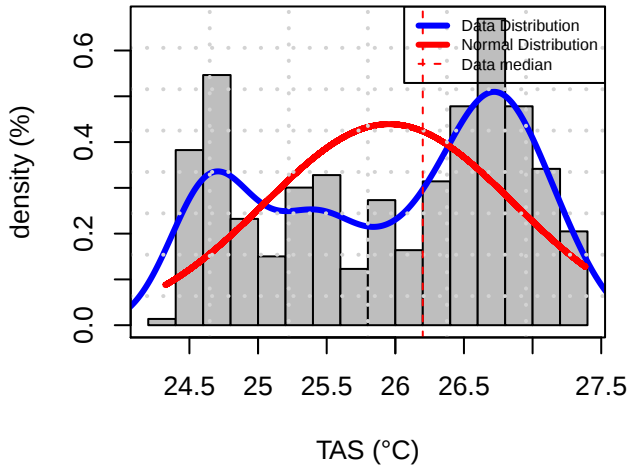
Histogram Distribution (TRTR)
