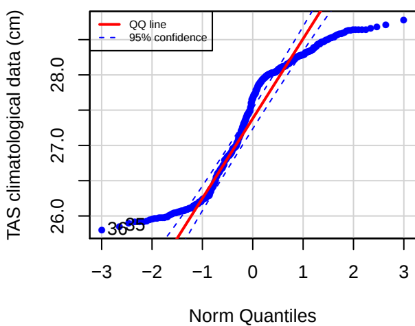
QQ plot (VCLC)
