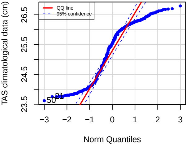
QQ plot (VCLR)
