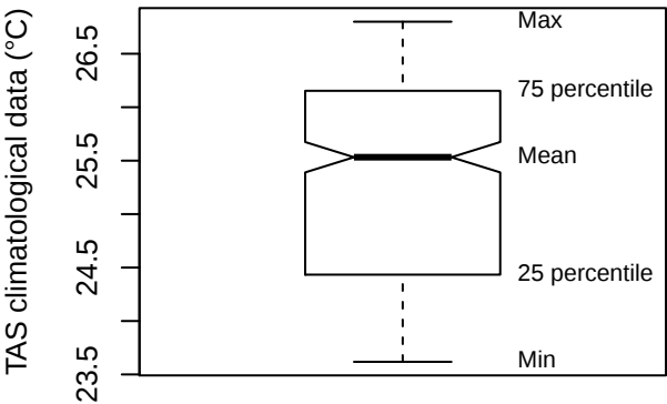
Box plot (VCLR)
