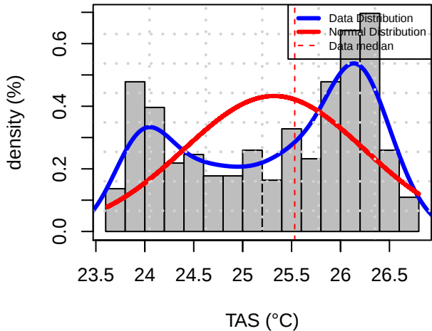
Histogram Distribution (VCLR)
