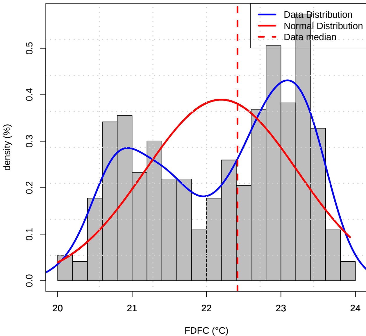
Histogram of Data distribution (TAS of FDFC)
