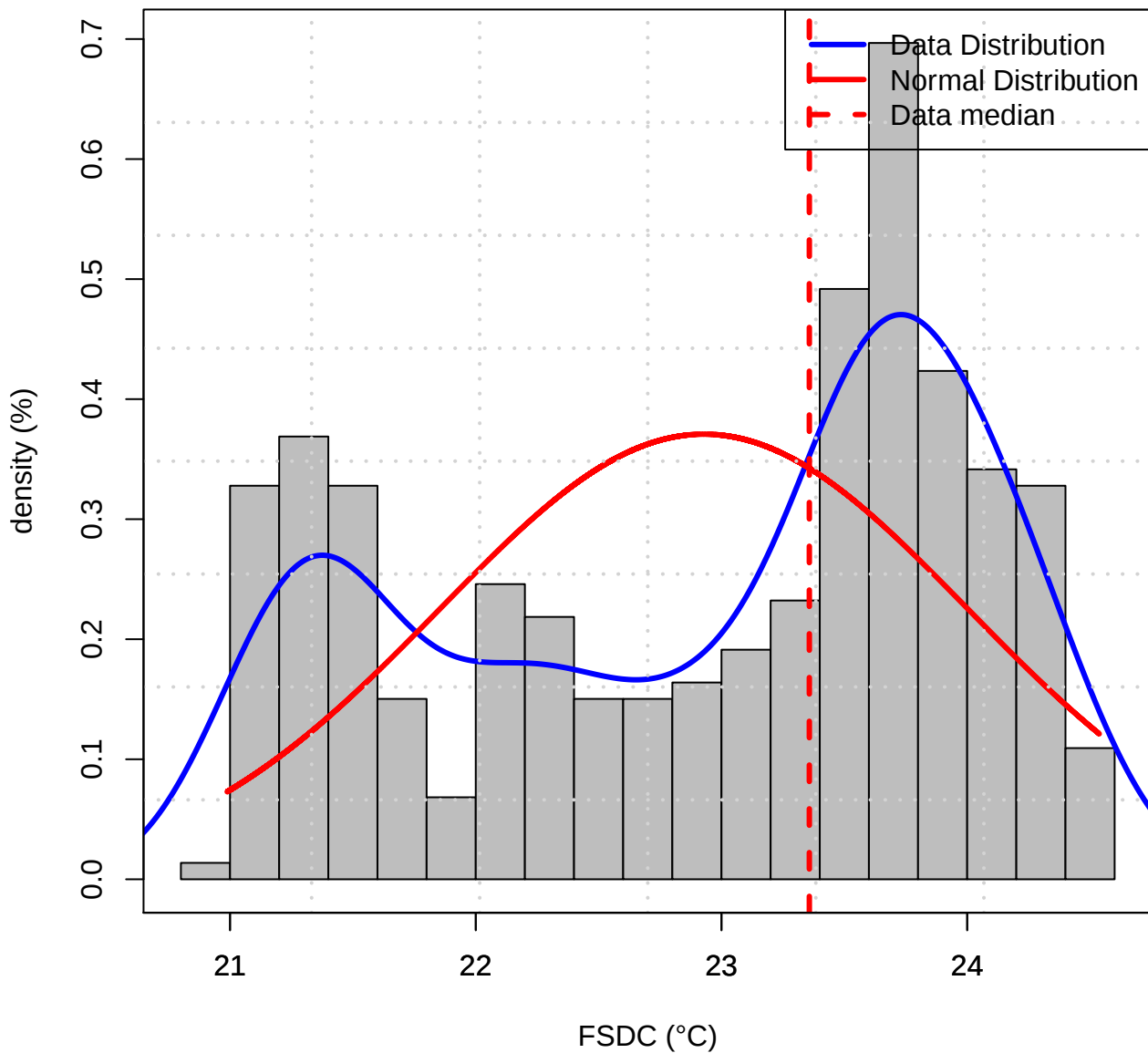
Histogram of Data distribution (TAS of FSDC)
