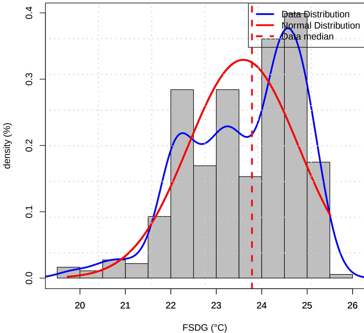
Histogram of Data distribution (TAS of FSDG)
