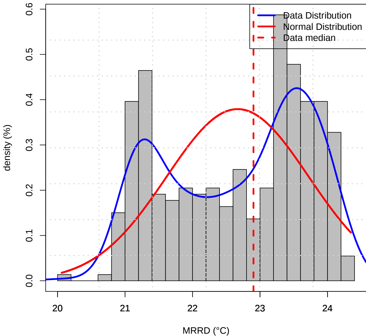
Histogram of Data distribution (TAS of MRRD)
