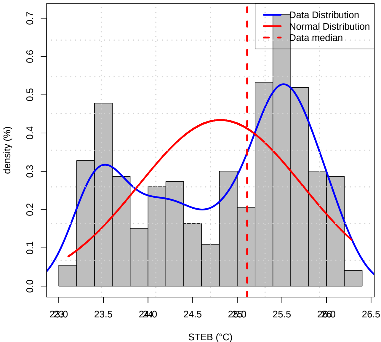
Histogram of Data distribution (TAS of STEB)
