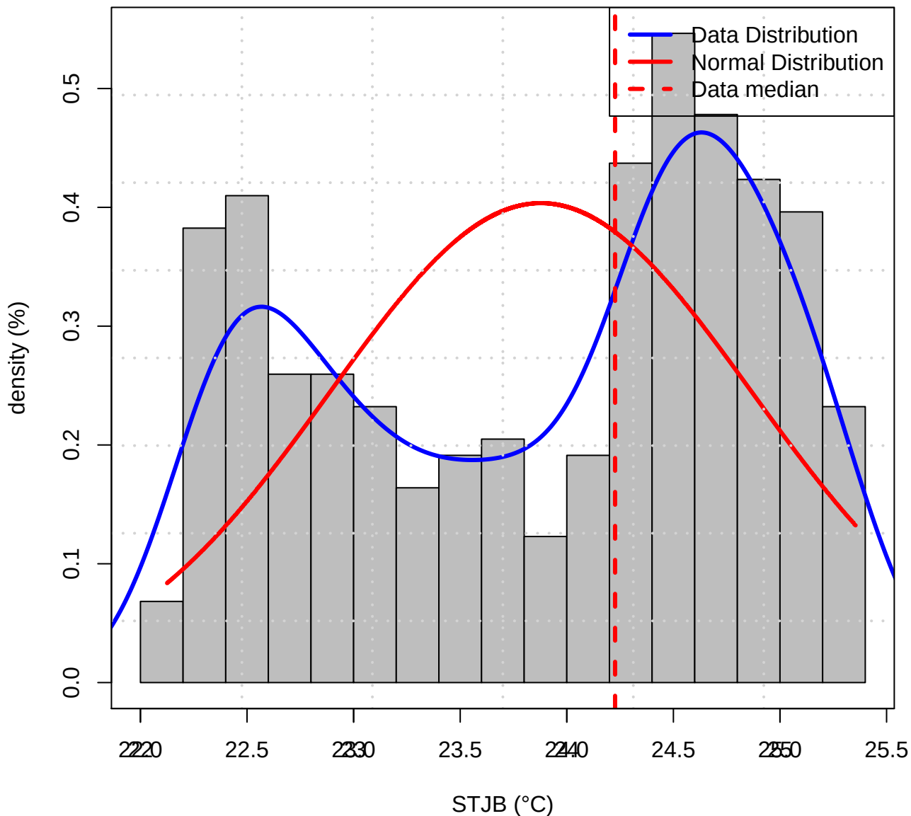
Histogram of Data distribution (TAS of STJB)
