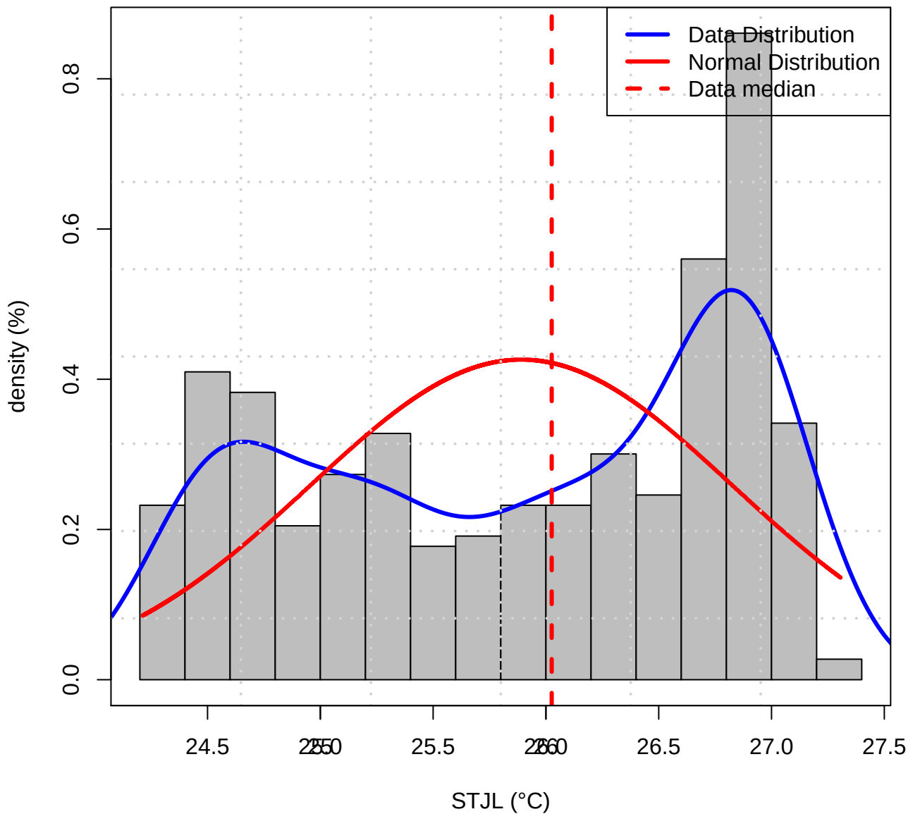
Histogram of Data distribution (TAS of STJL)
