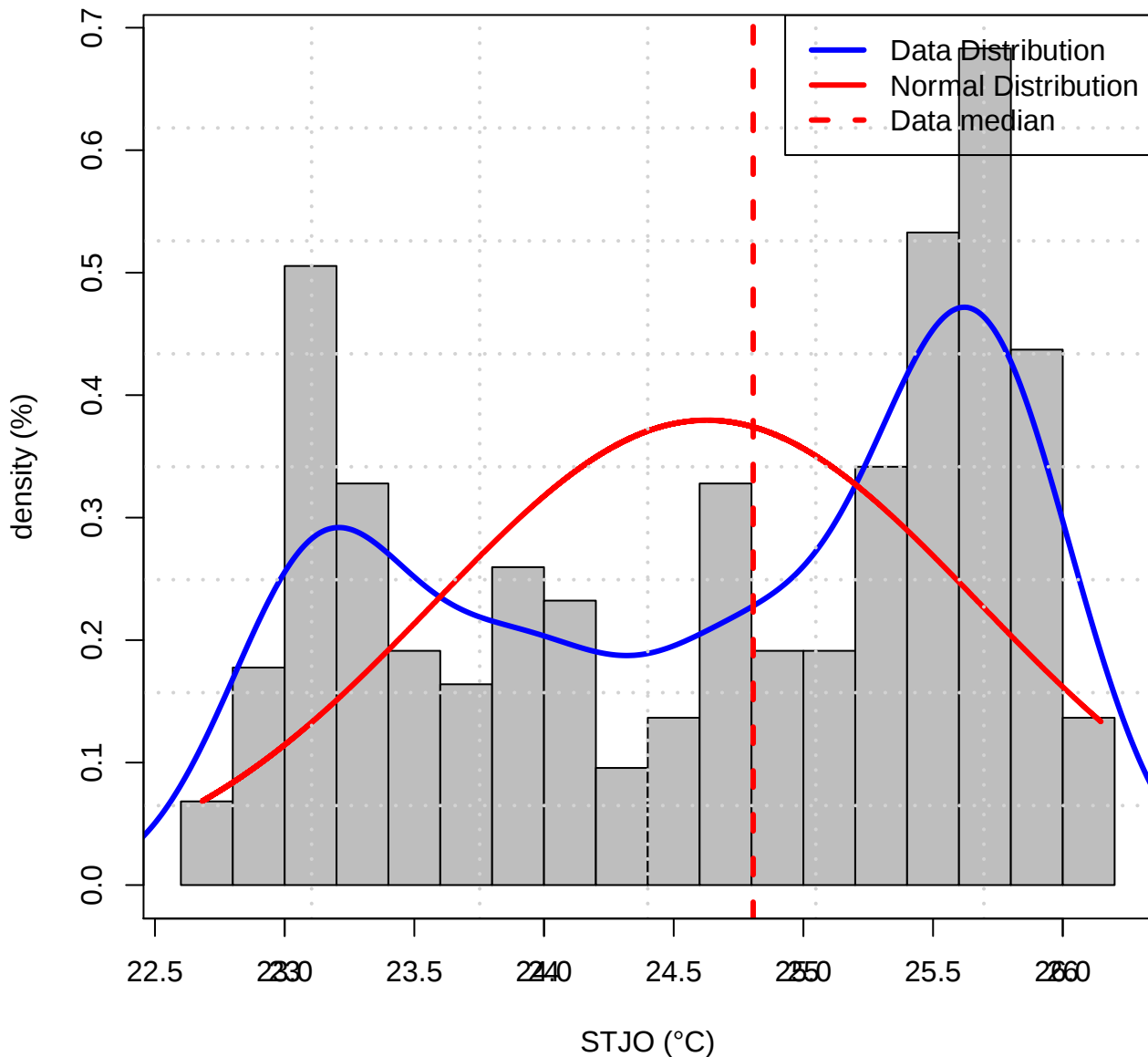
Histogram of Data distribution (TAS of STJO)
