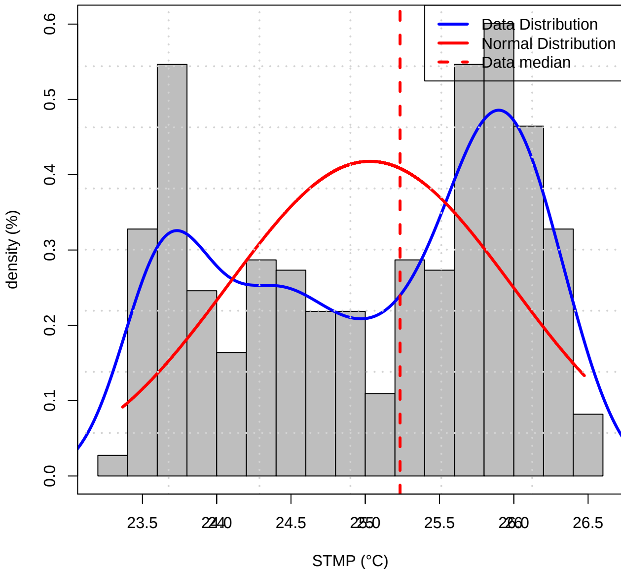
Histogram of Data distribution (TAS of STMP)
