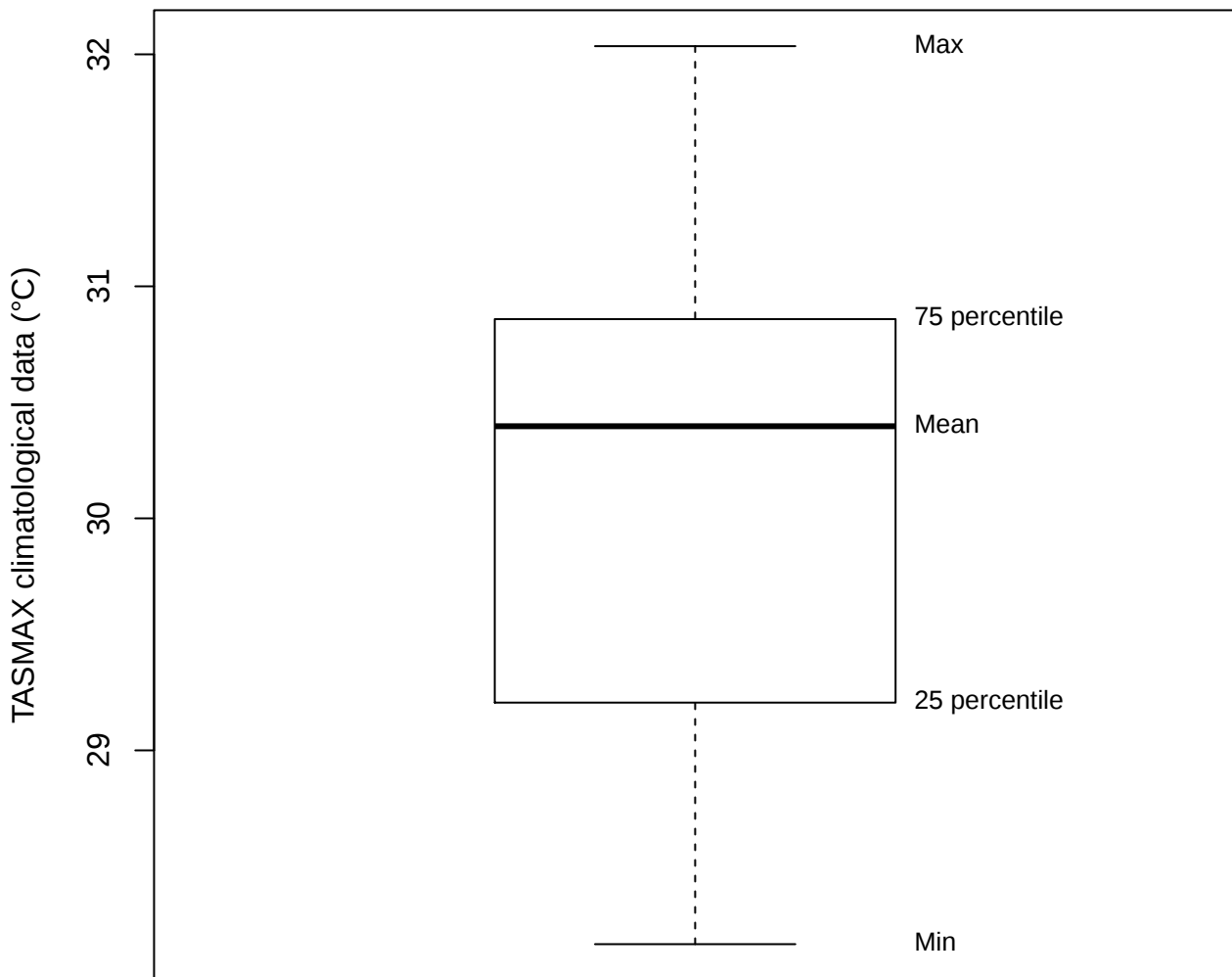
Box plot (TAS of DUCO)
