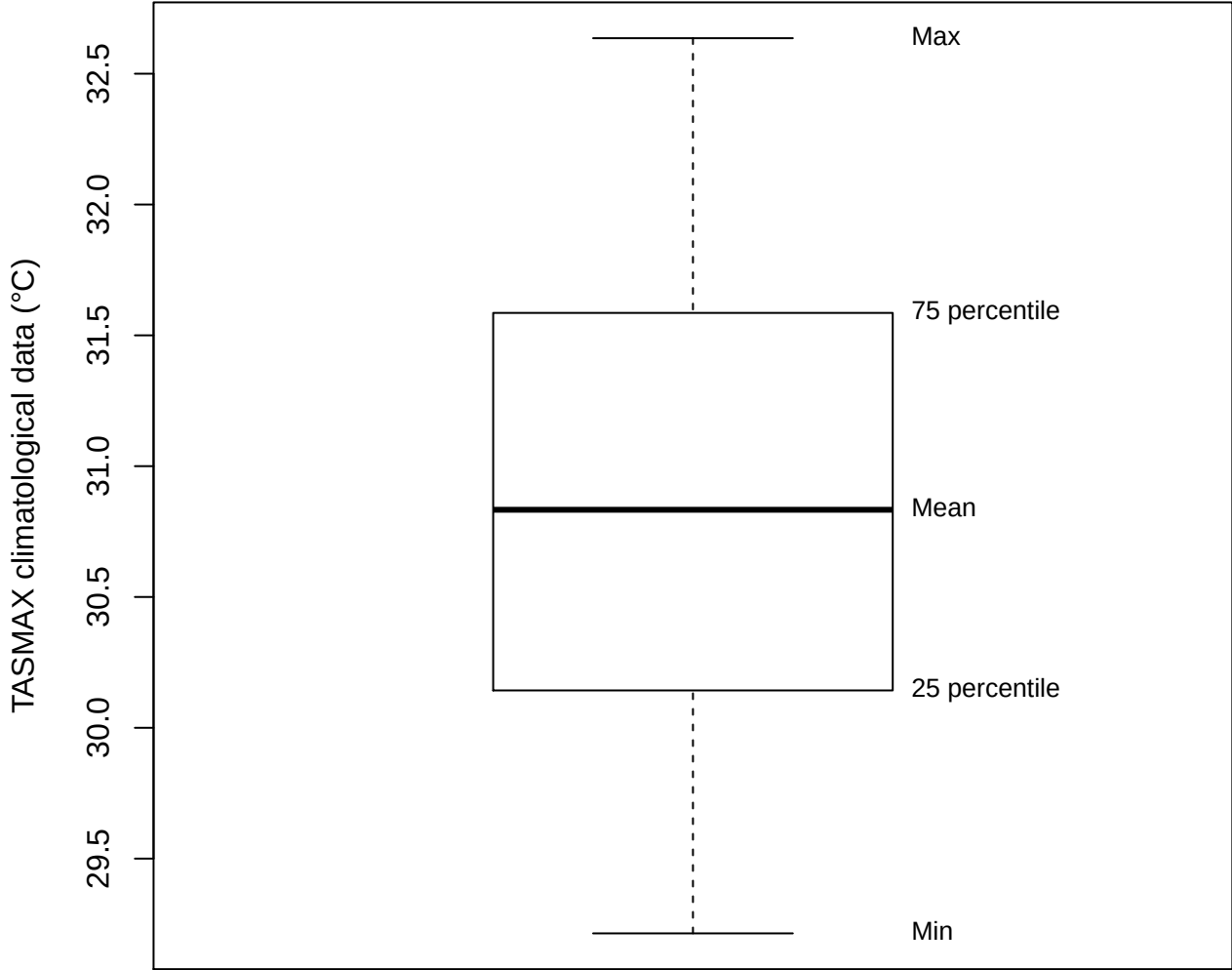
Box plot (TAS of ROBP)
