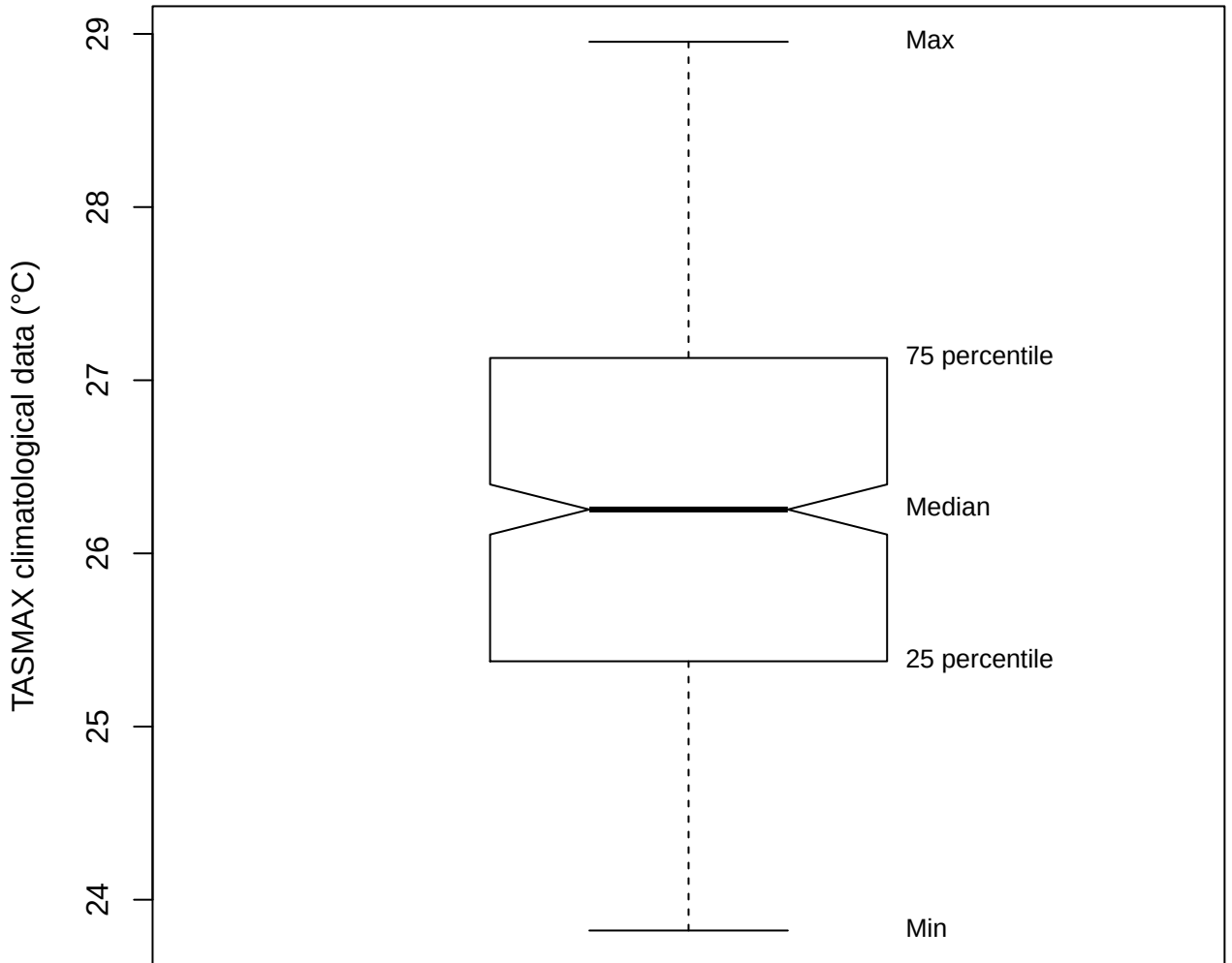
Box plot (TASMAX of BLLF)
