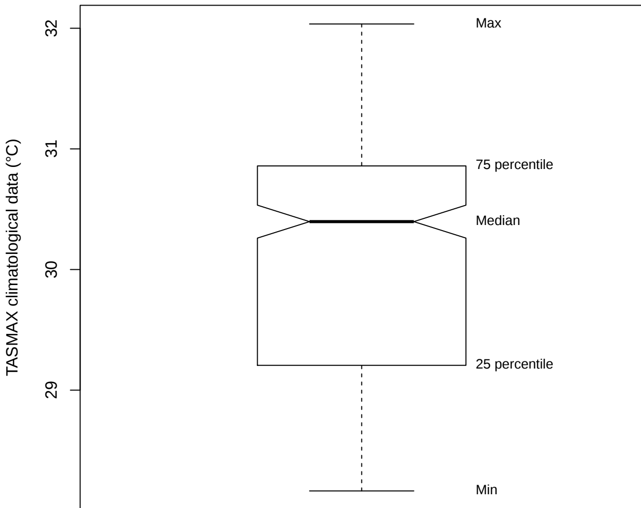
Box plot (TASMAX of DUCO)
