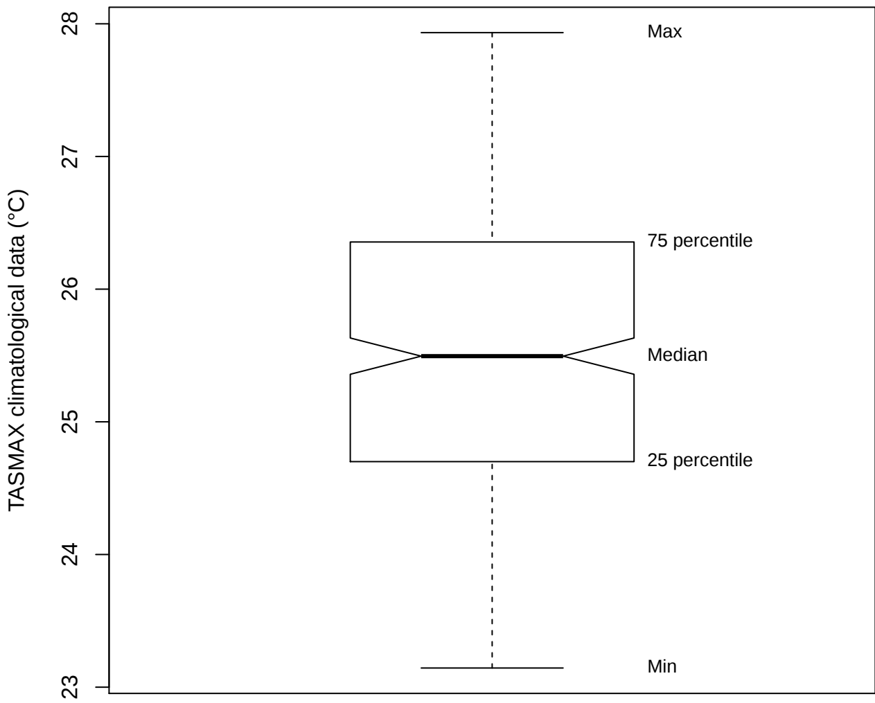
Box plot (TASMAX of FDFC)
