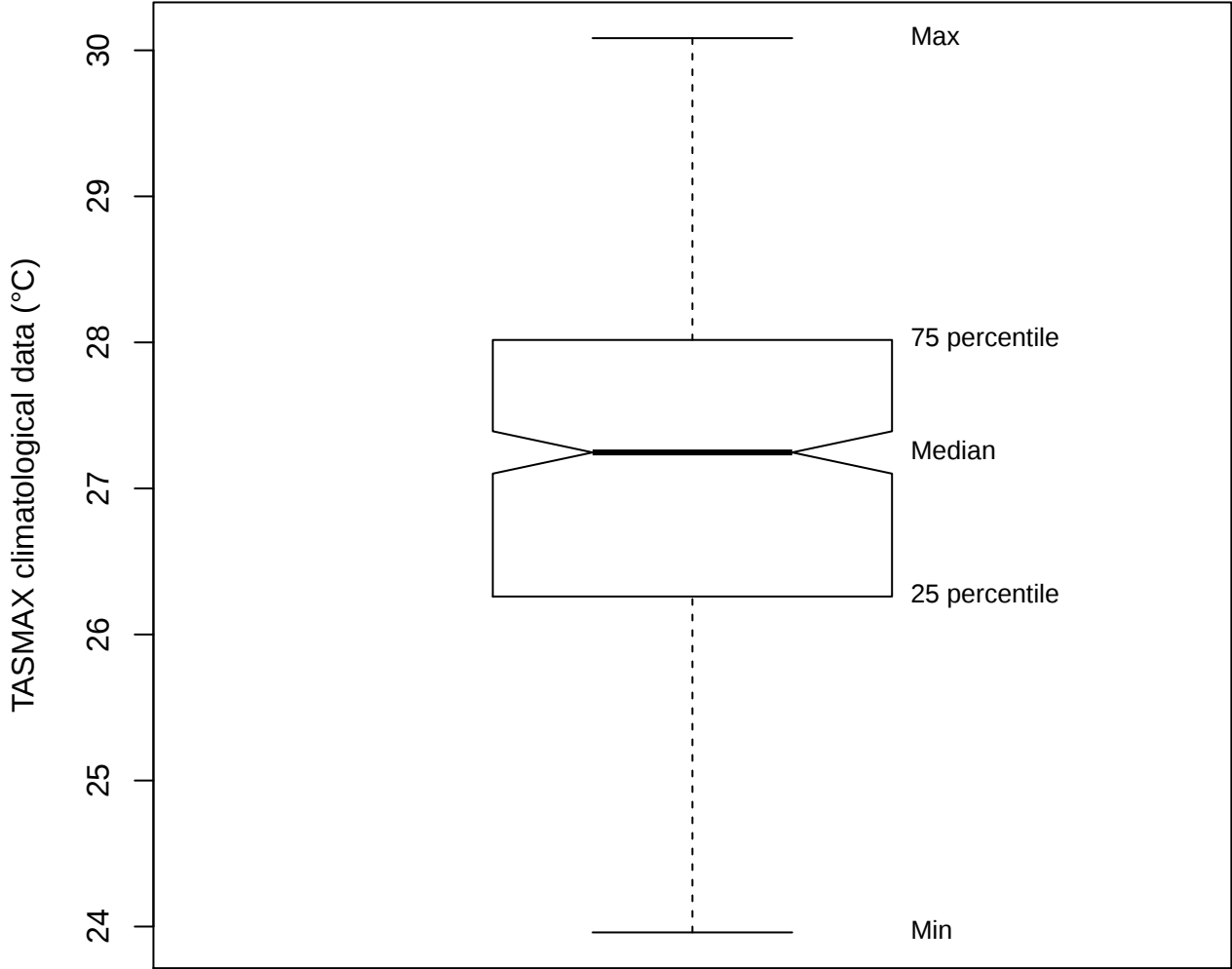
Box plot (TASMAX of FSDG)
