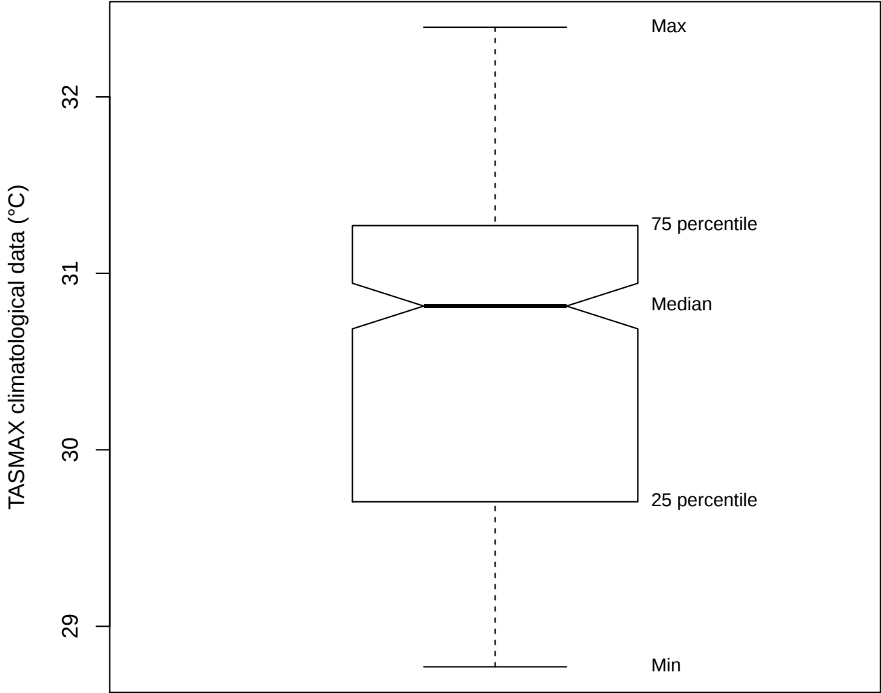
Box plot (TASMAX of LAMA)
