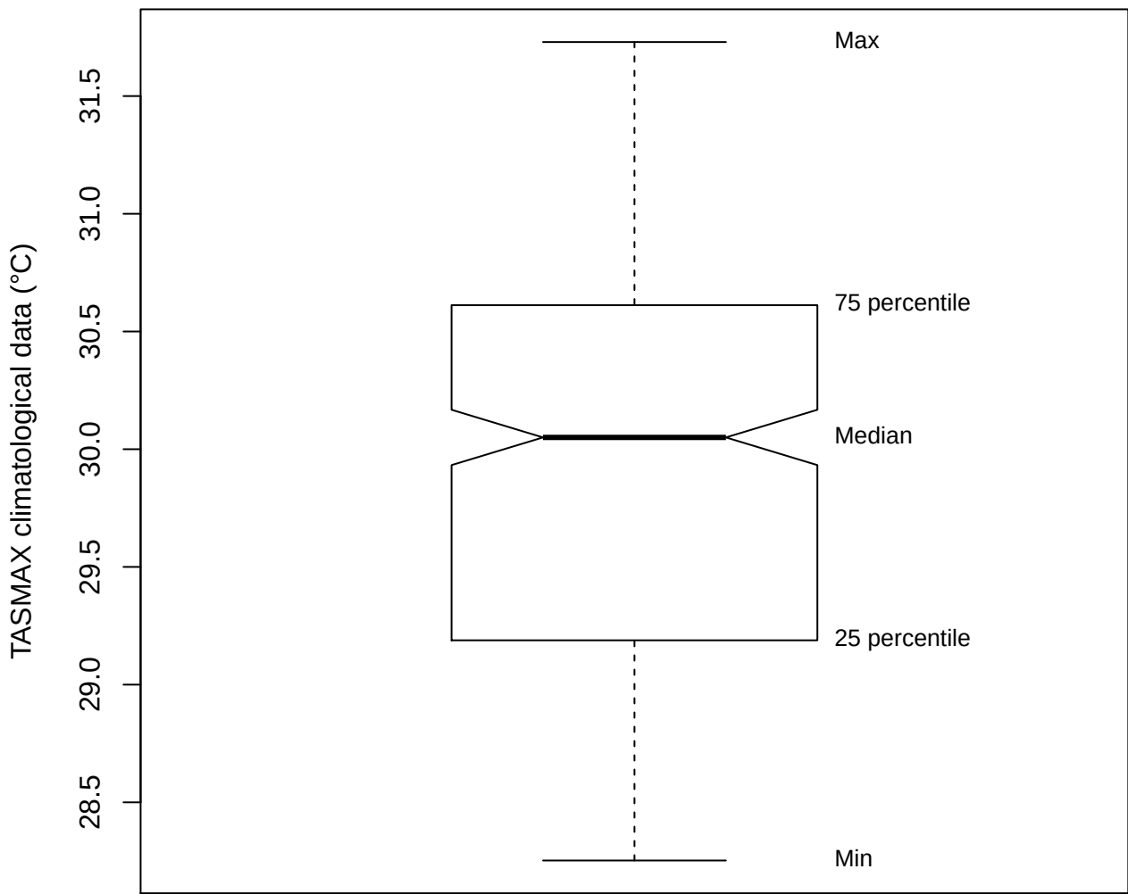
Box plot (TASMAX of LFRC)
