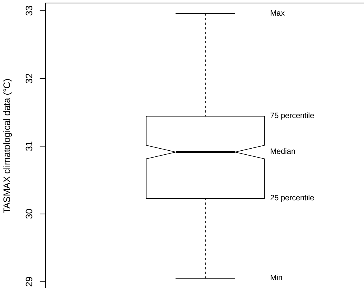
Box plot (TASMAX of LFRS)
