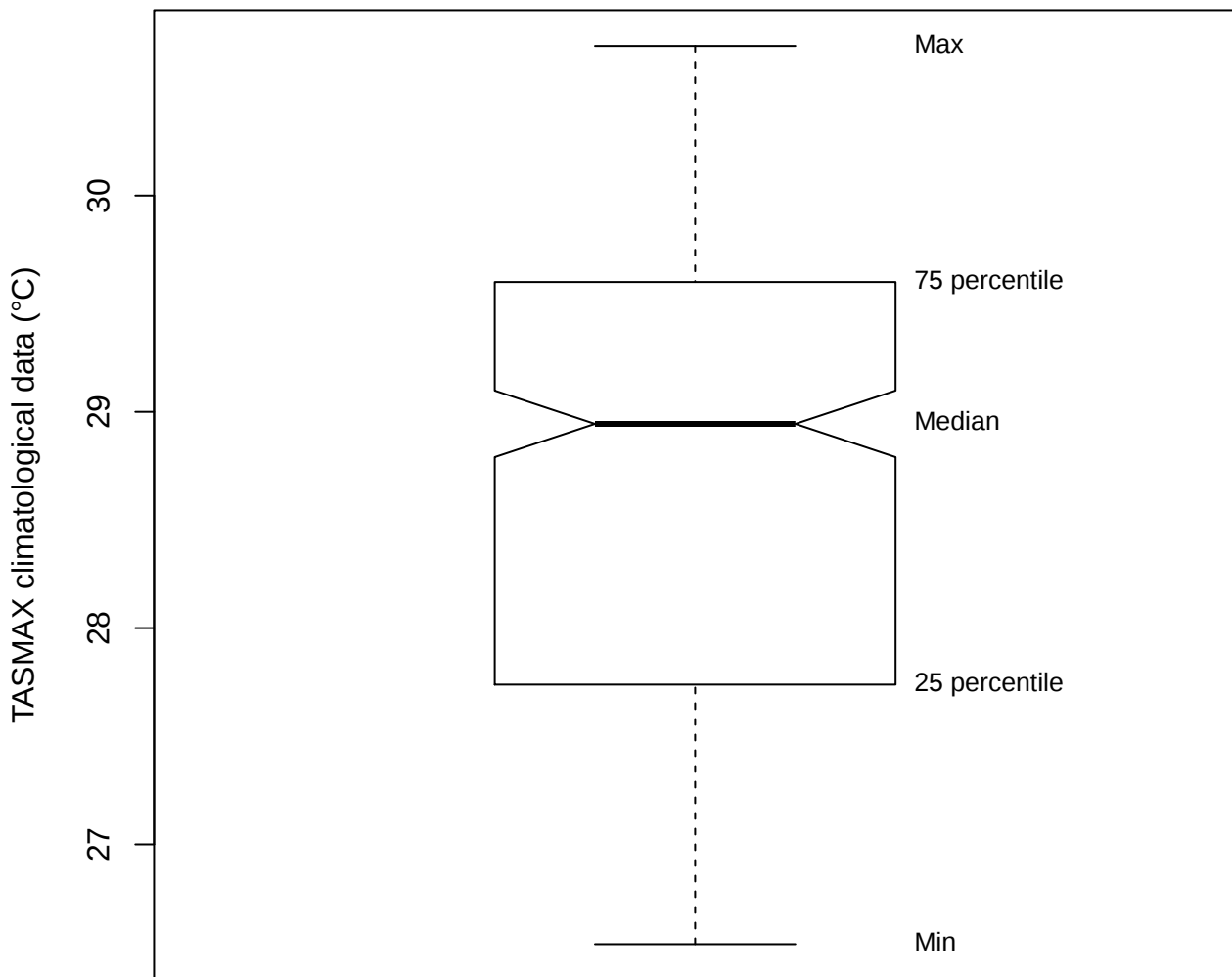
Box plot (TASMAX of MARB)
