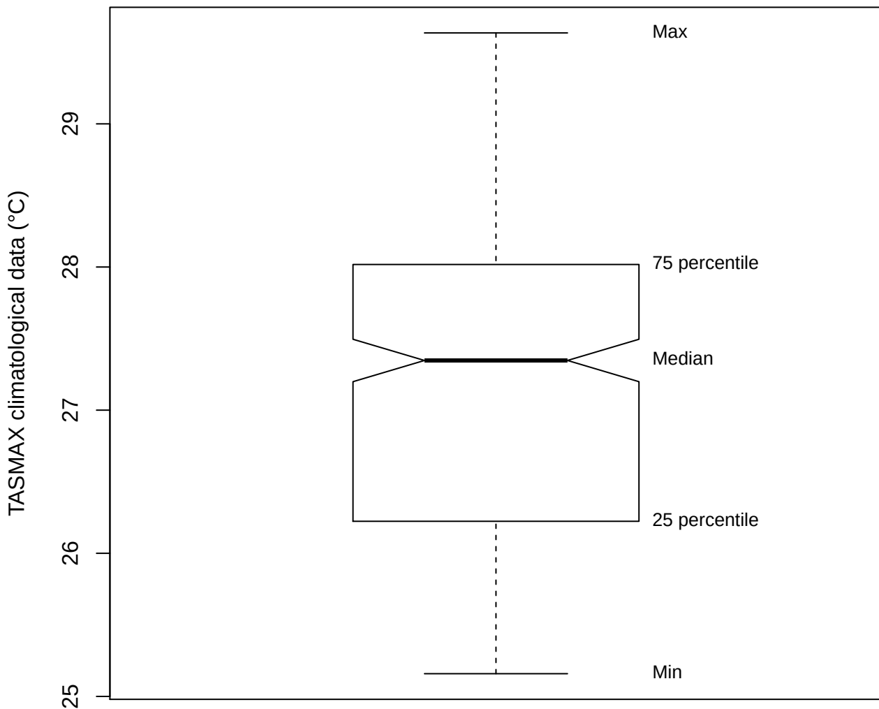
Box plot (TASMAX of MRRC)
