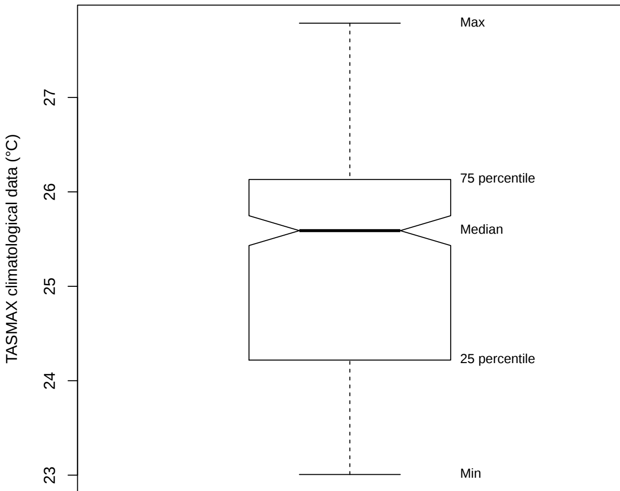
Box plot (TASMAX of MRRD)
