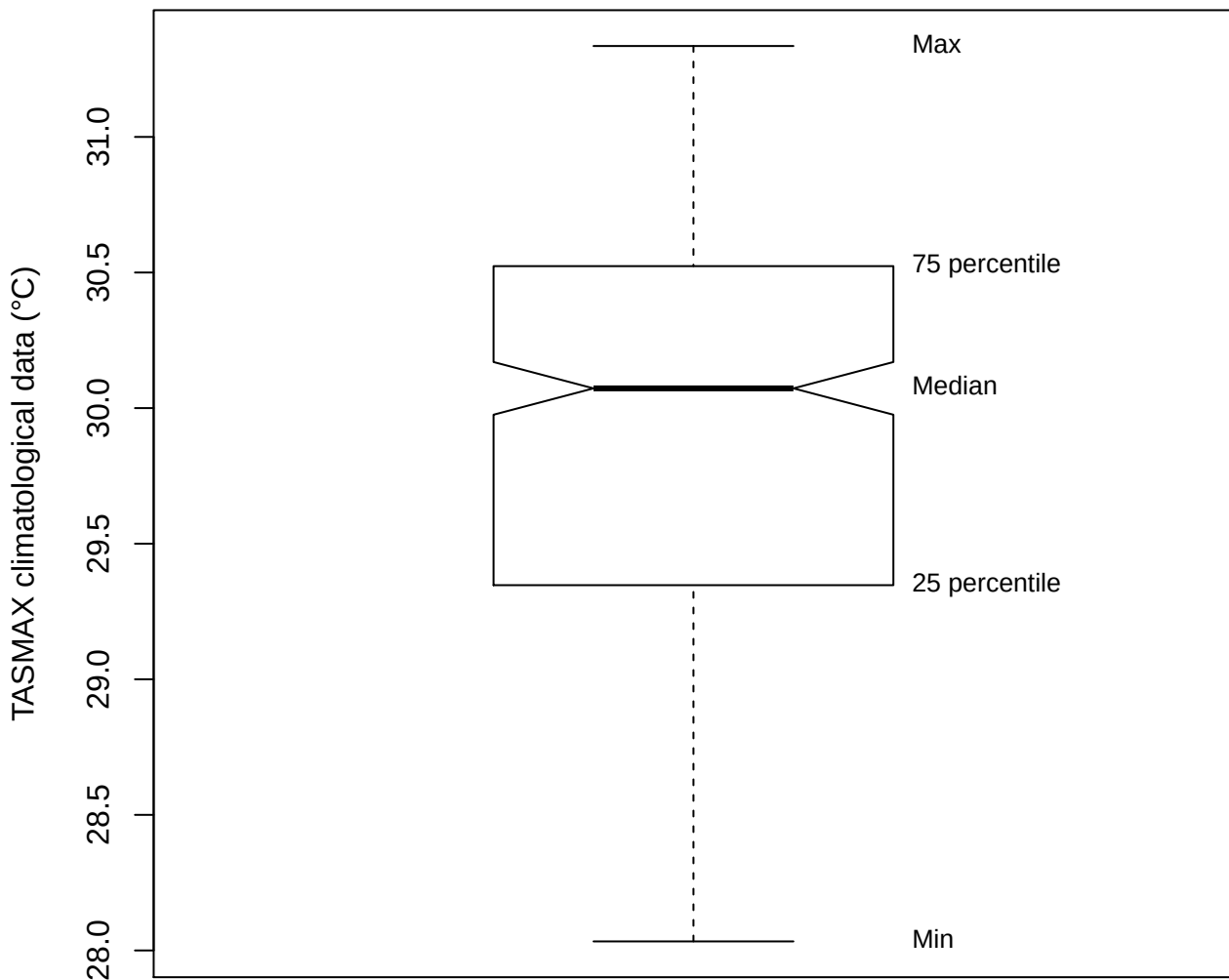
Box plot (TASMAX of STAN)
