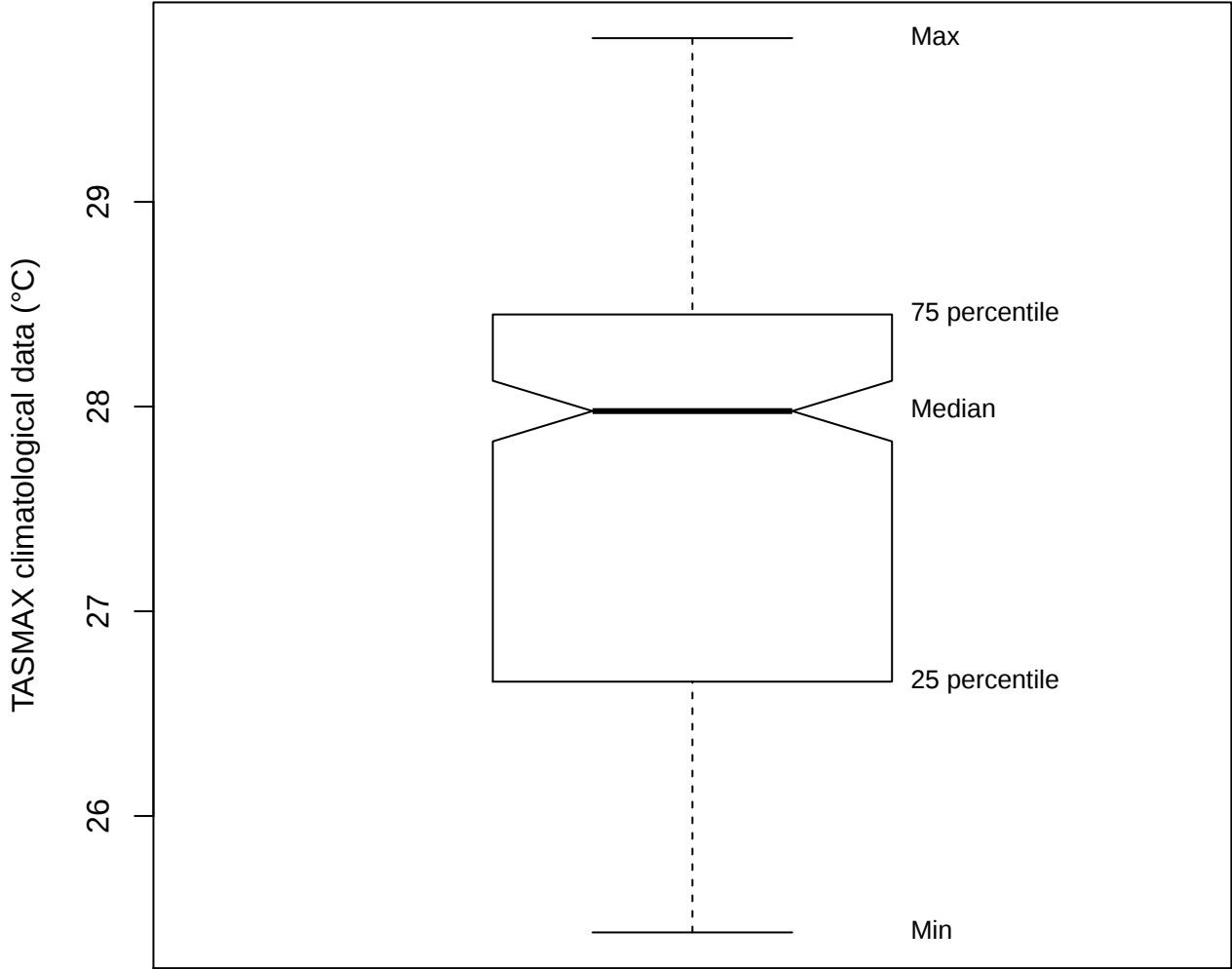
Box plot (TASMAX of STEB)
