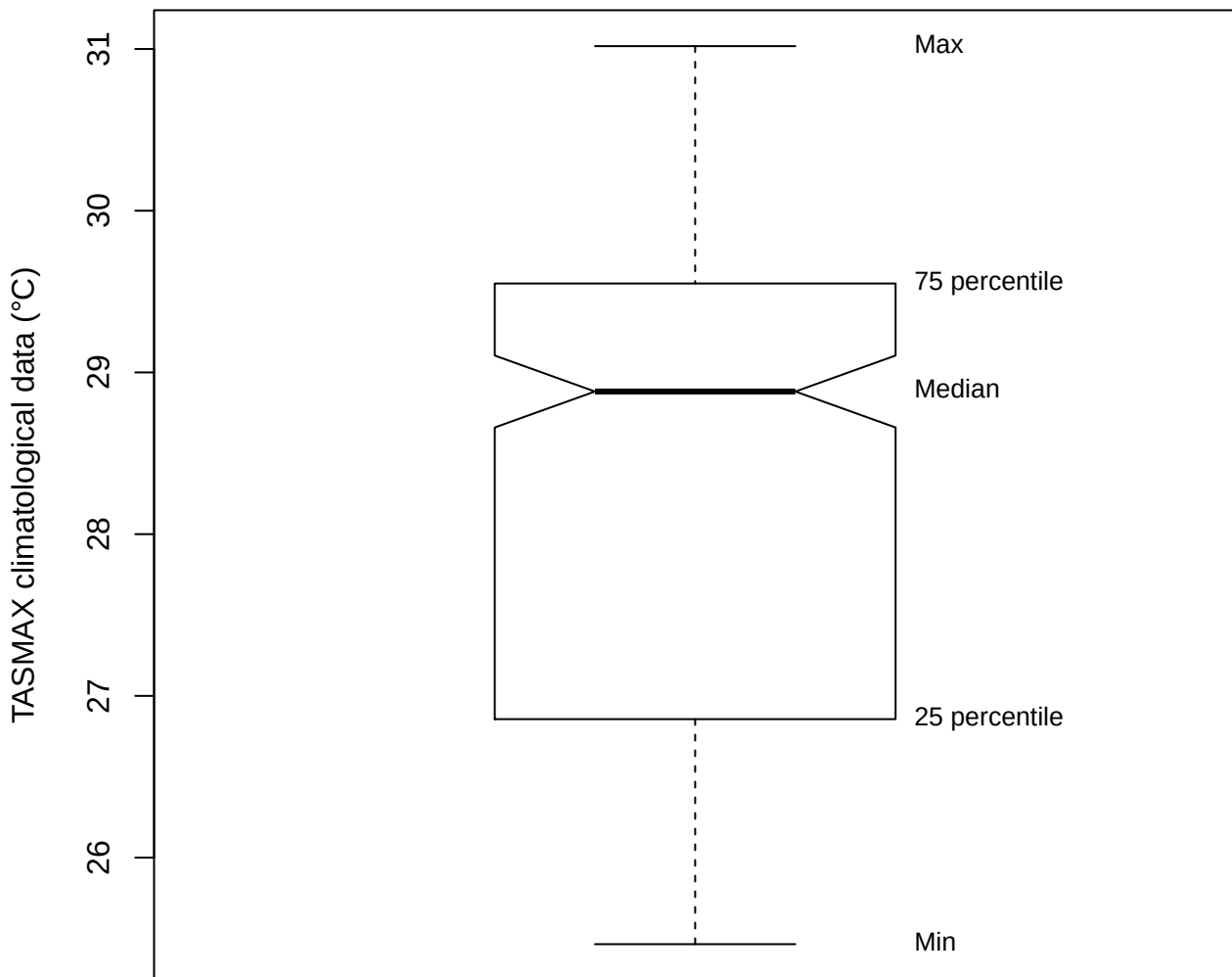
Box plot (TASMAX of STJO)
