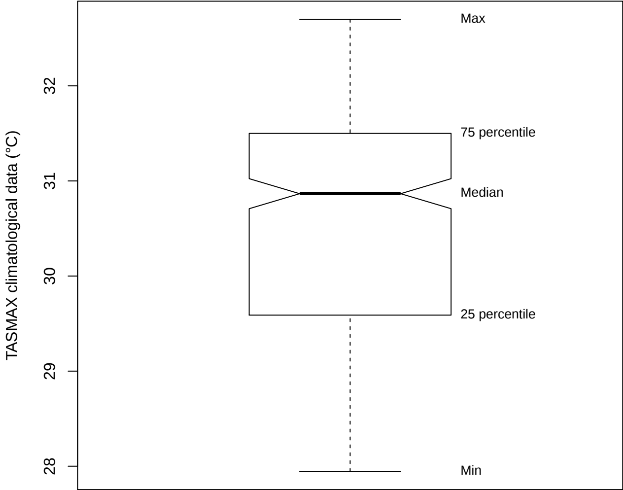
Box plot (TASMAX of STMB)
