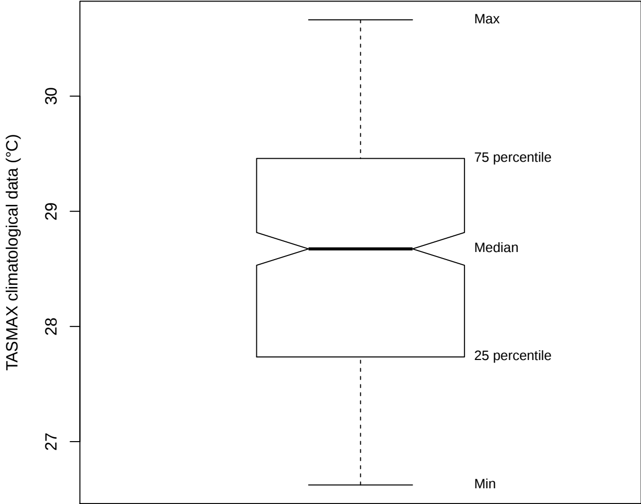
Box plot (TASMAX of STMP)
