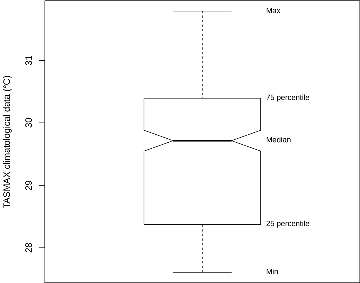
Box plot (TASMAX of TRTC)
