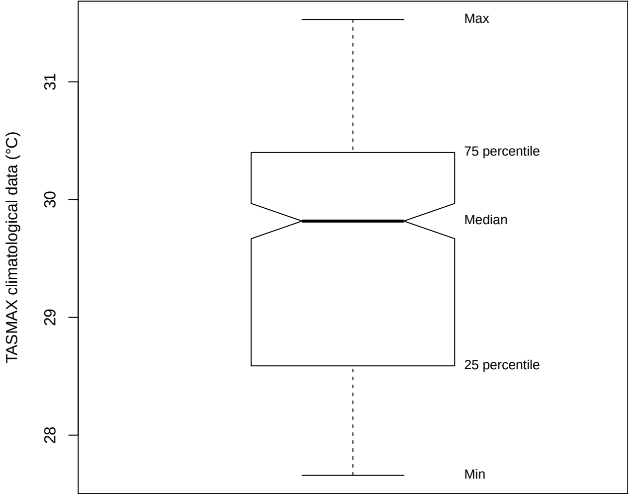
Box plot (TASMAX of VCLC)
