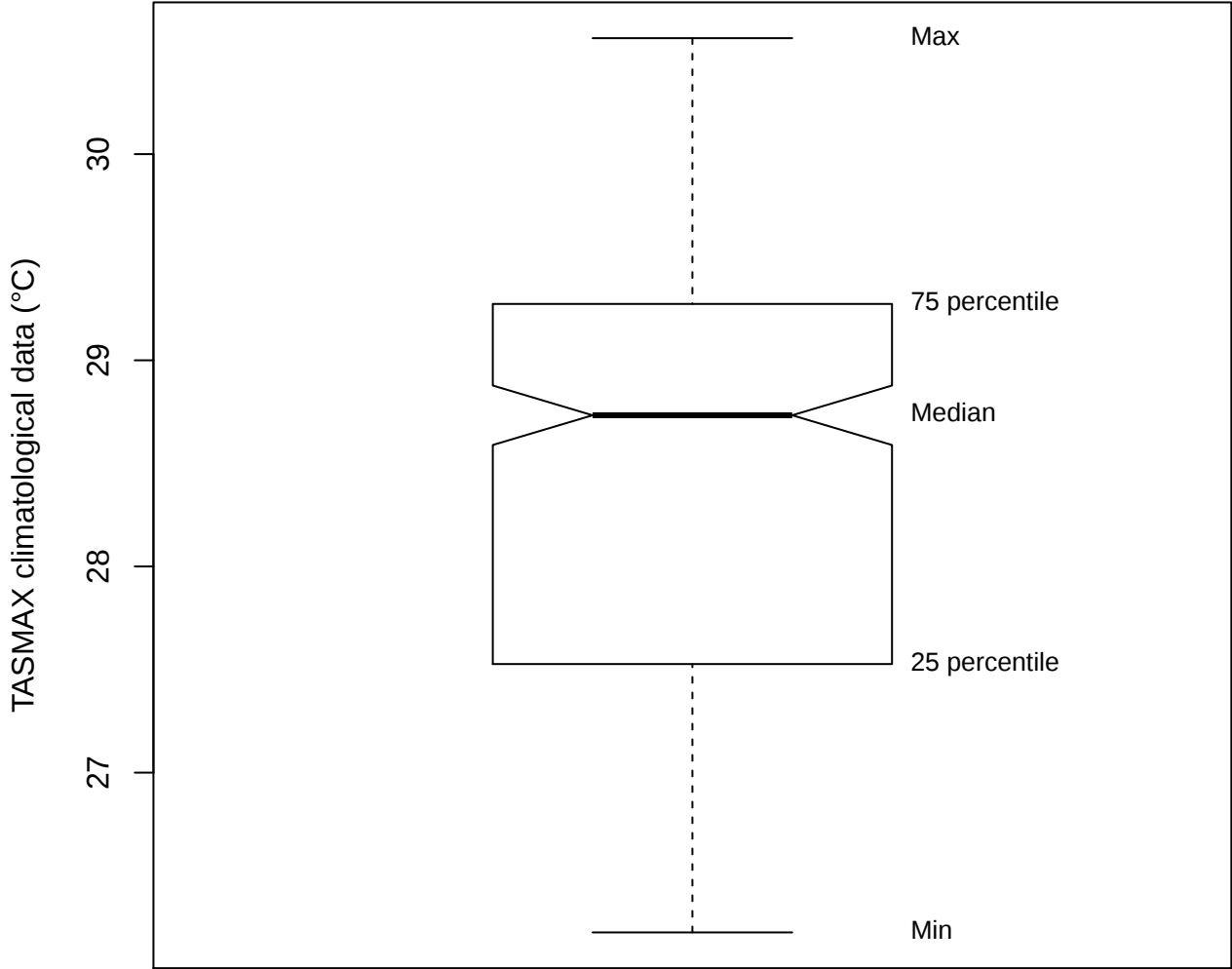
Box plot (TASMAX of VCLR)
