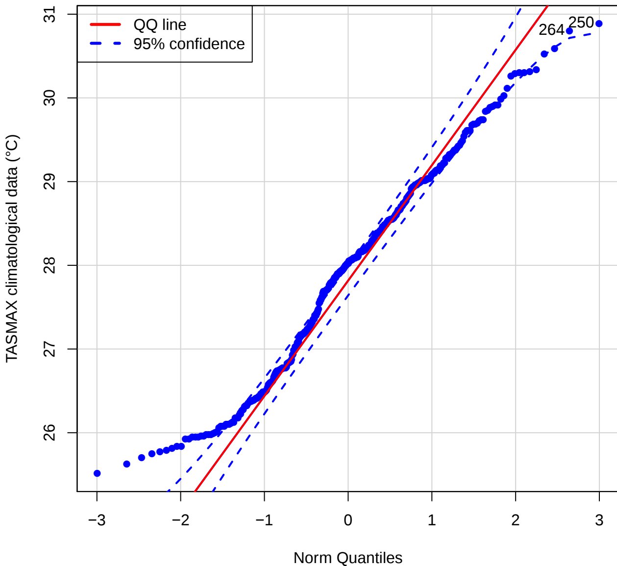
QQ plot (TASMAX of AJPB)
