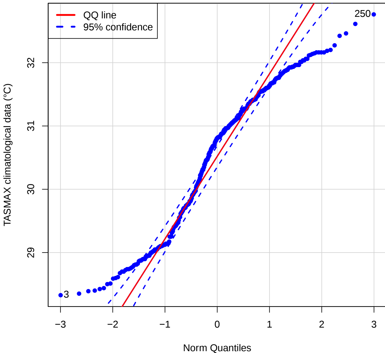
QQ plot (TASMAX of BASP)
