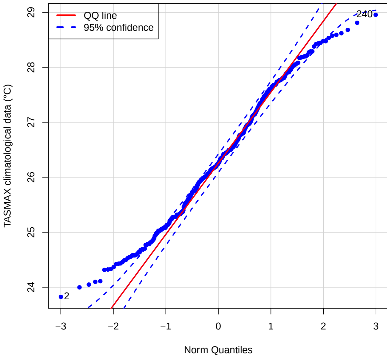
QQ plot (TASMAX of BLLF)
