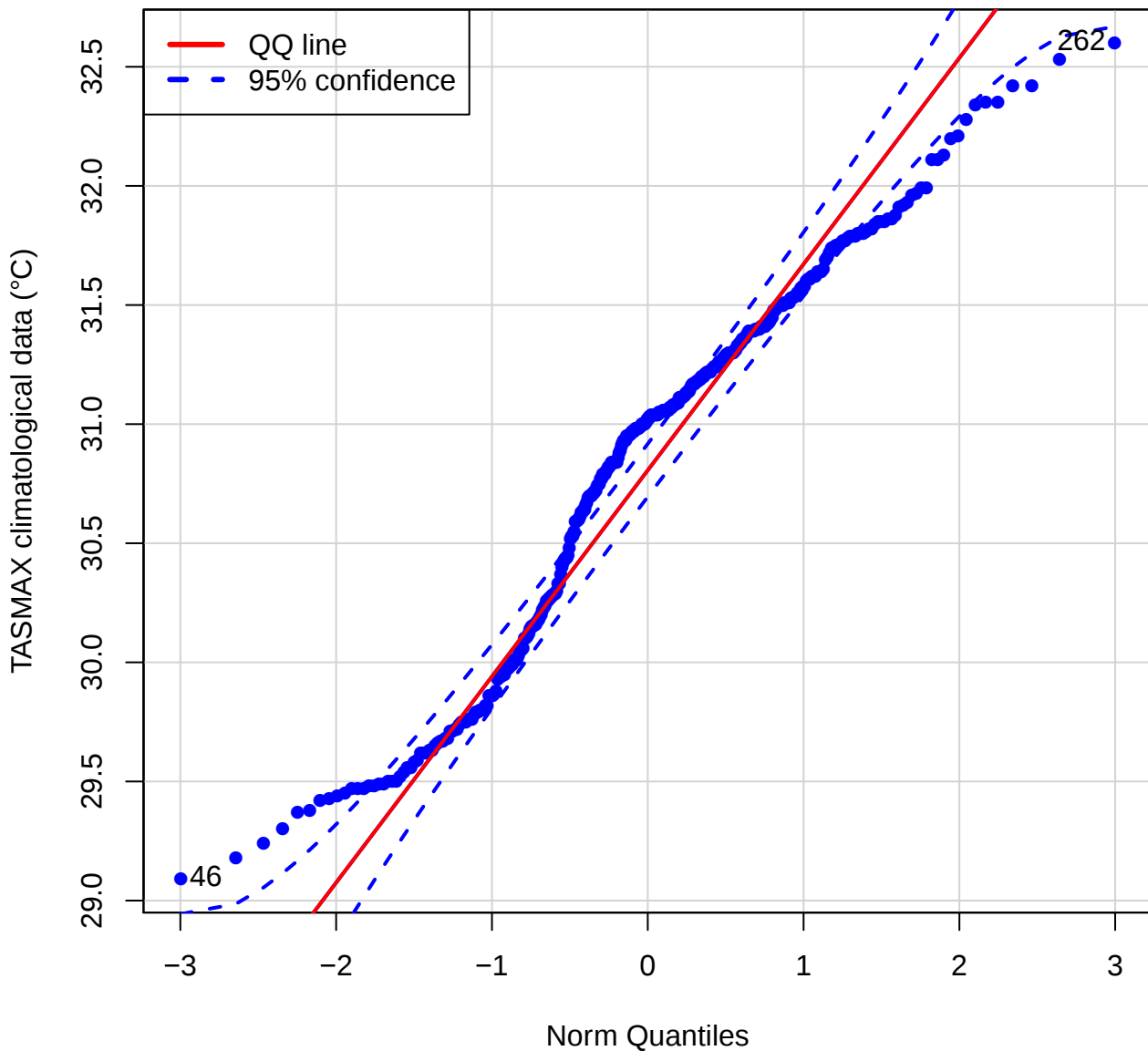
QQ plot (TASMAX of DIAM)
