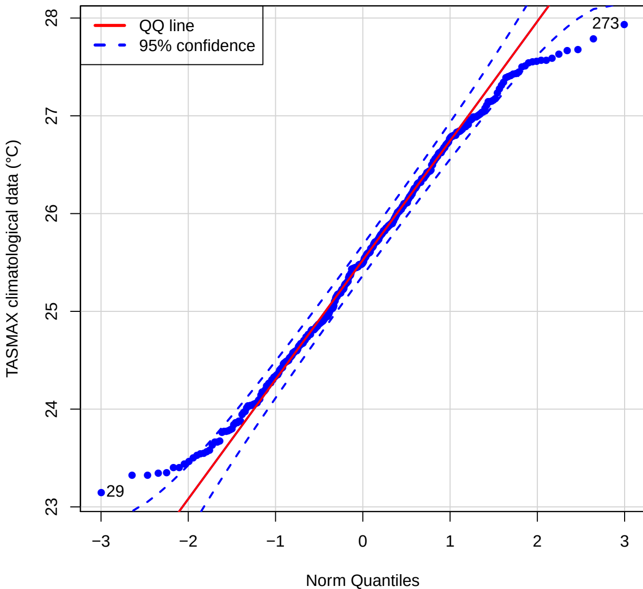
QQ plot (TASMAX of FDFC)
