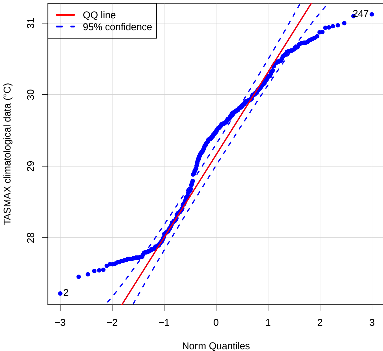
QQ plot (TASMAX of FDFD)
