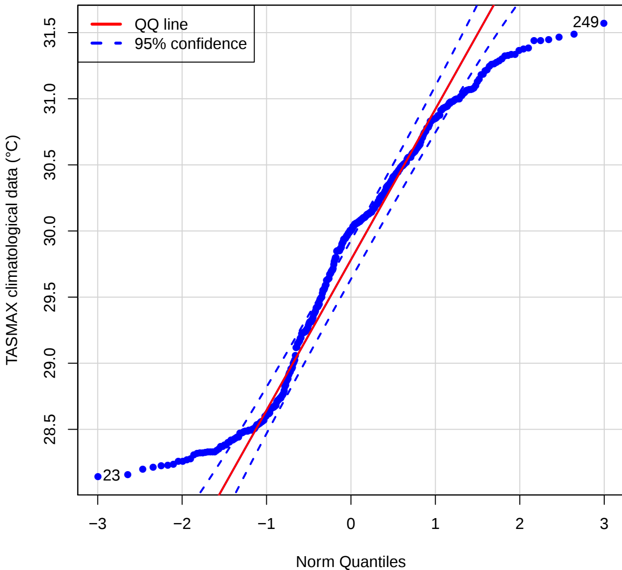
QQ plot (TASMAX of FDFF)
