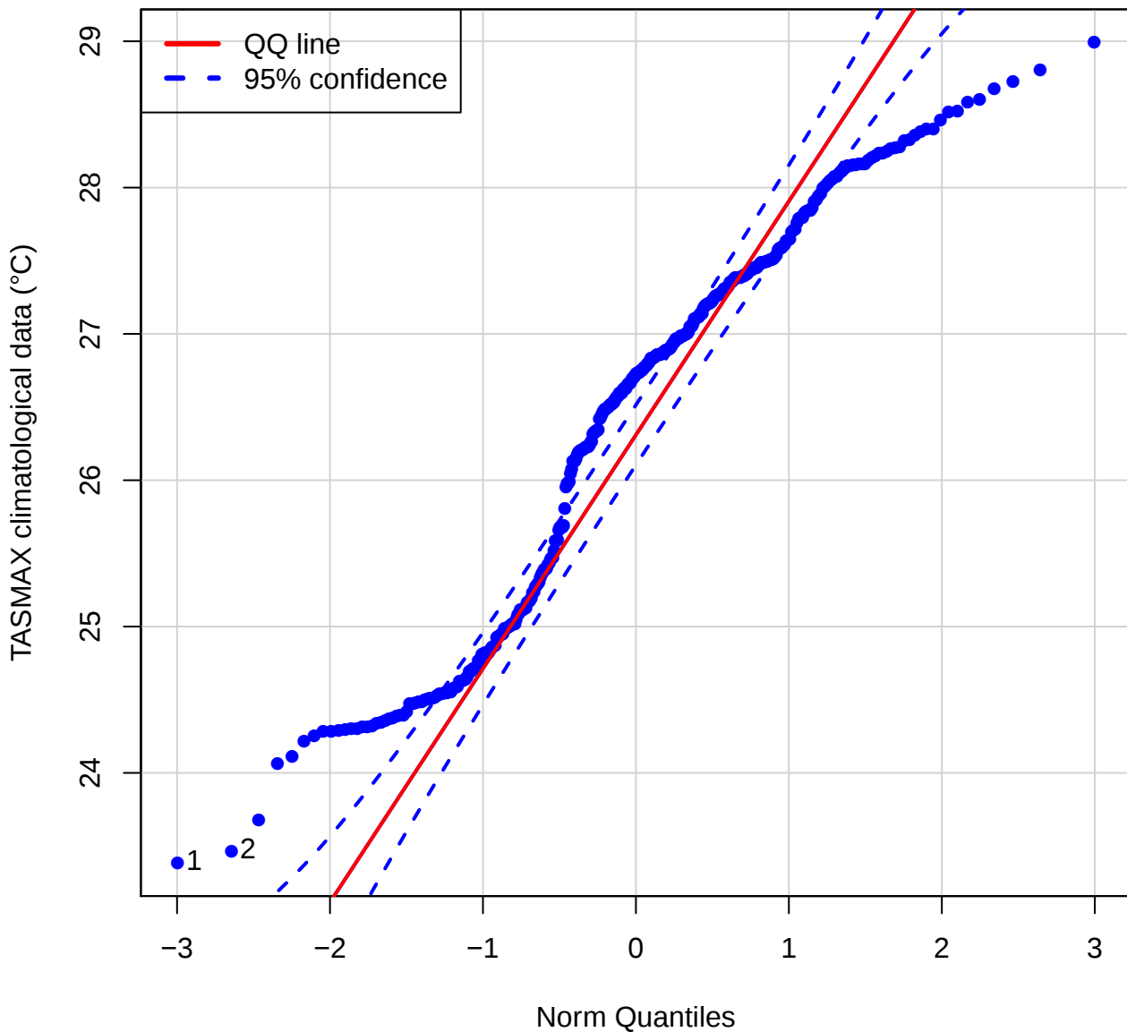
QQ plot (TASMAX of FSDC)
