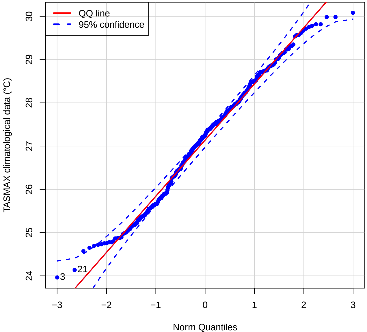
QQ plot (TASMAX of FSDG)
