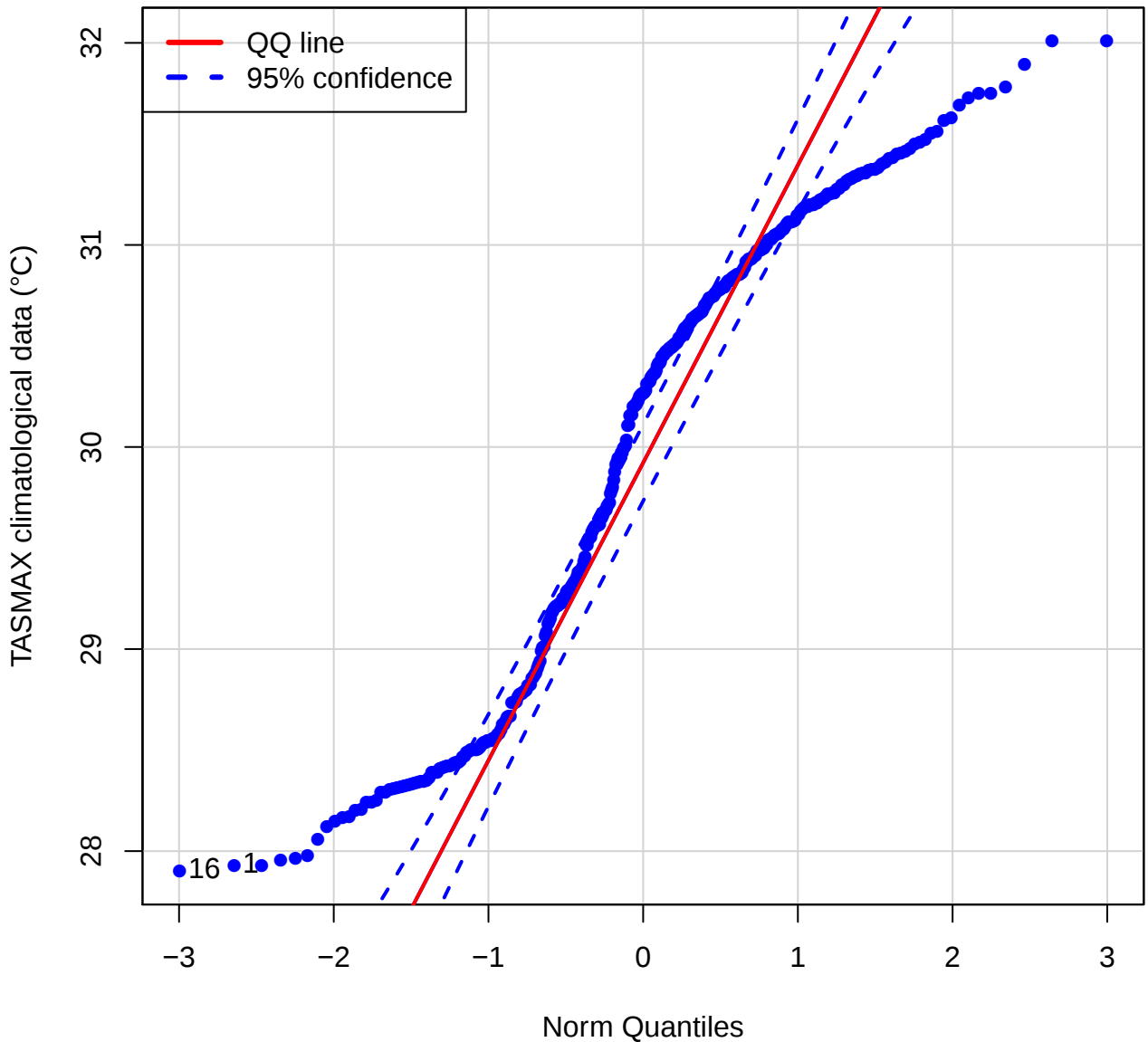
QQ plot (TASMAX of GDRV)
