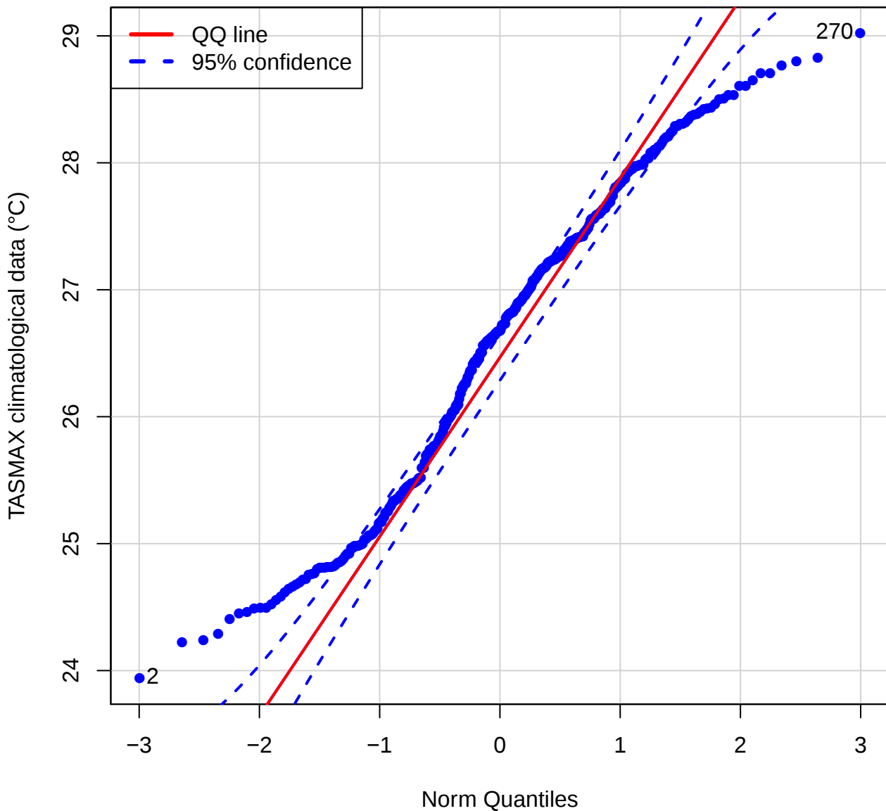
QQ plot (TASMAX of GMRN)
