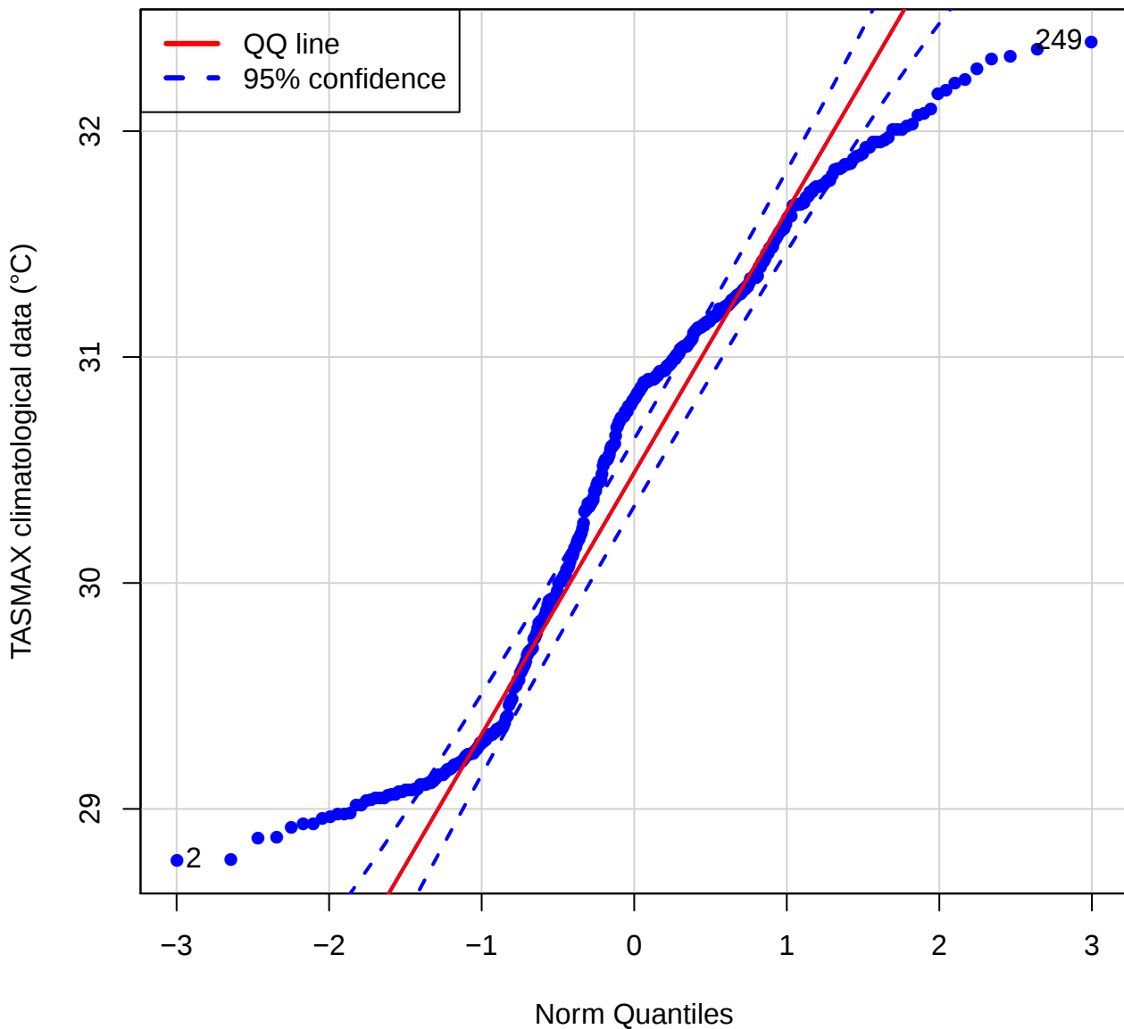
QQ plot (TASMAX of LAMA)
