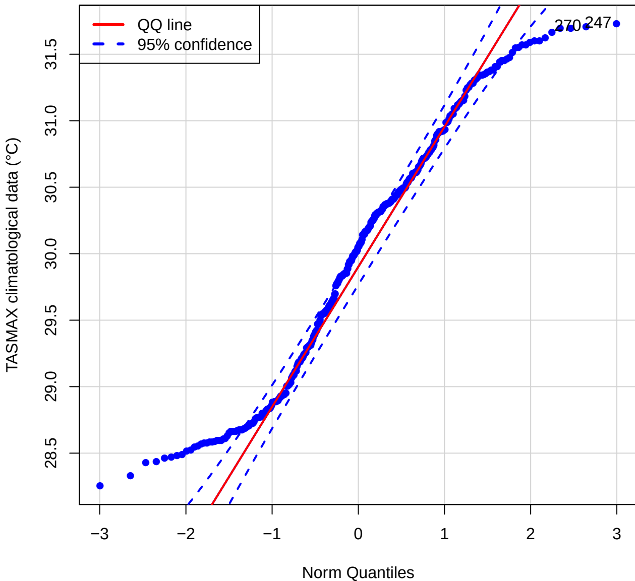
QQ plot (TASMAX of LFRC)
