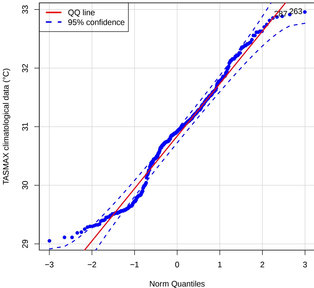
QQ plot (TASMAX of LFRS)
