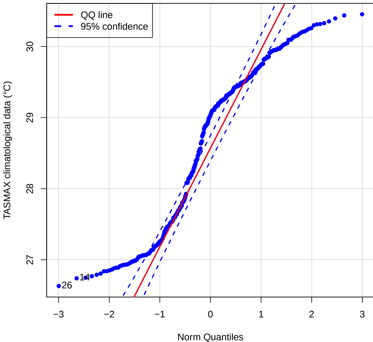
QQ plot (TASMAX of MACB)
