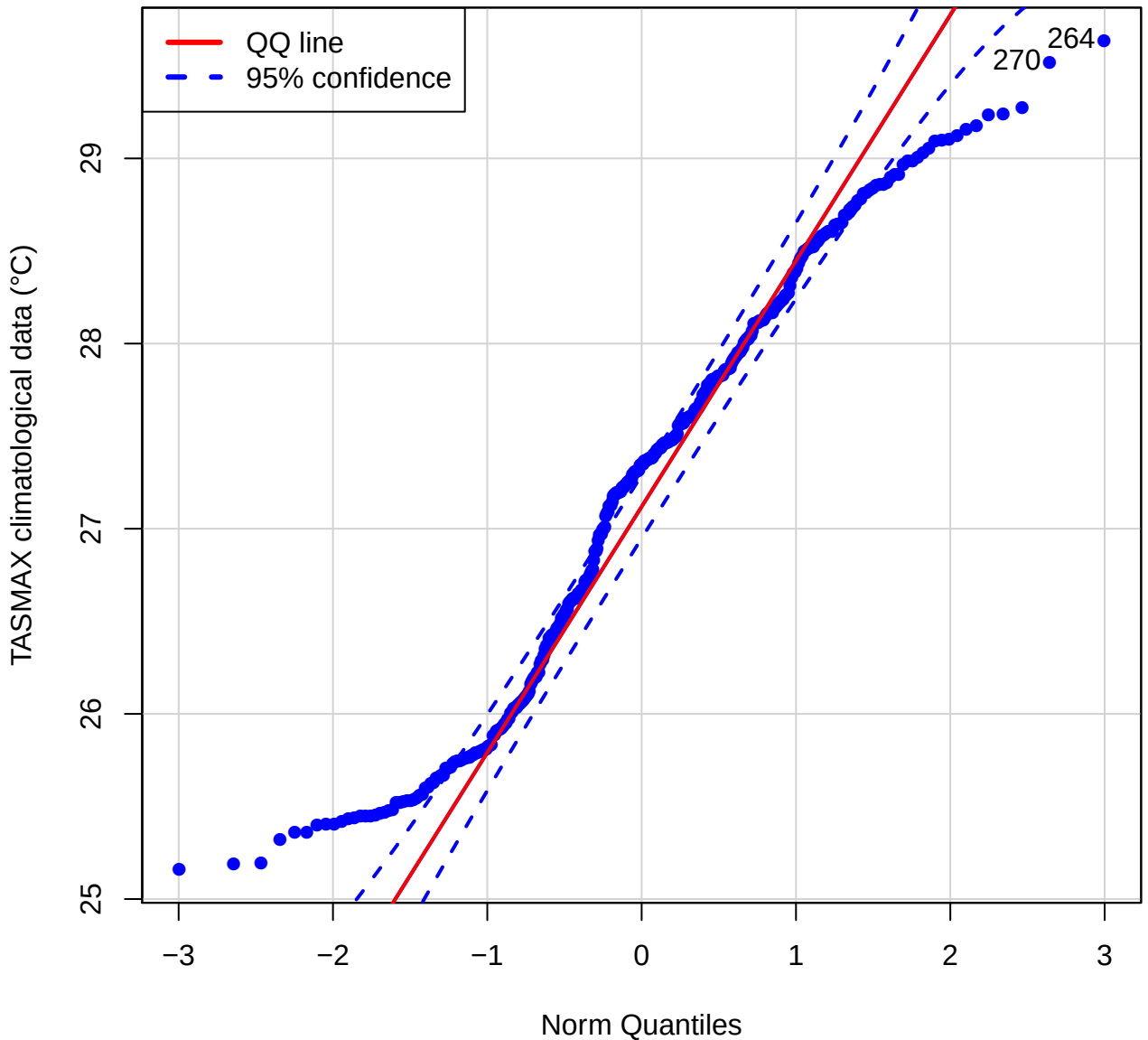
QQ plot (TASMAX of MRRC)
