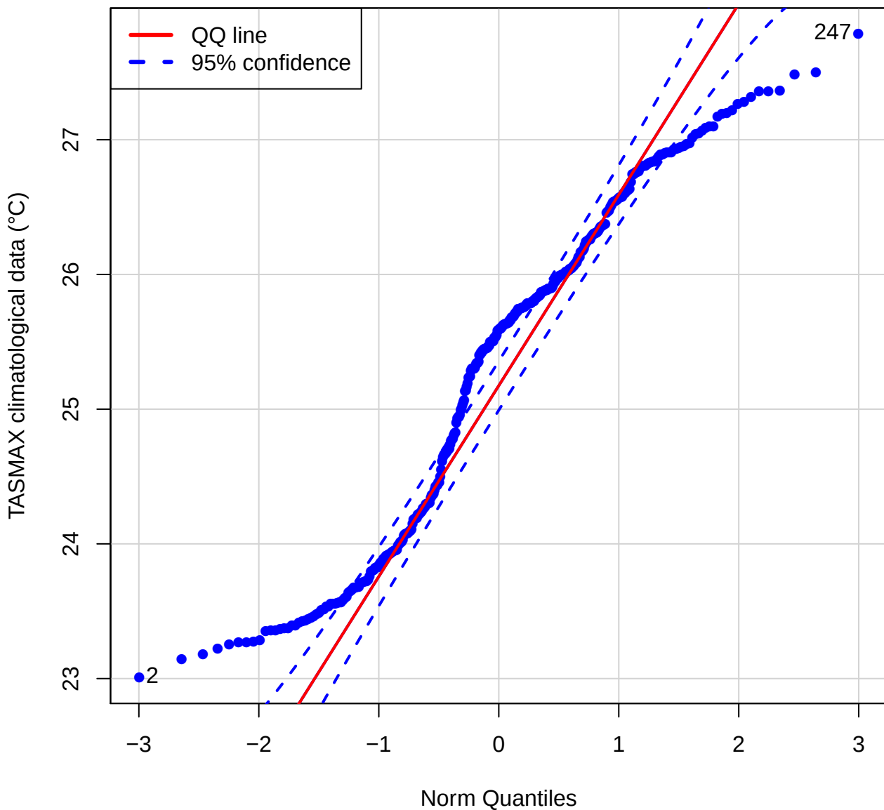
QQ plot (TASMAX of MRRD)
